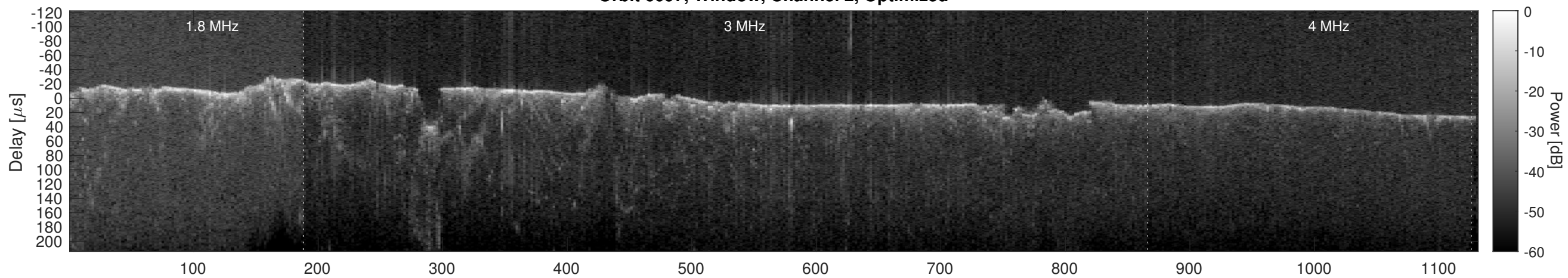
Orbit 6097, Cluttergram
