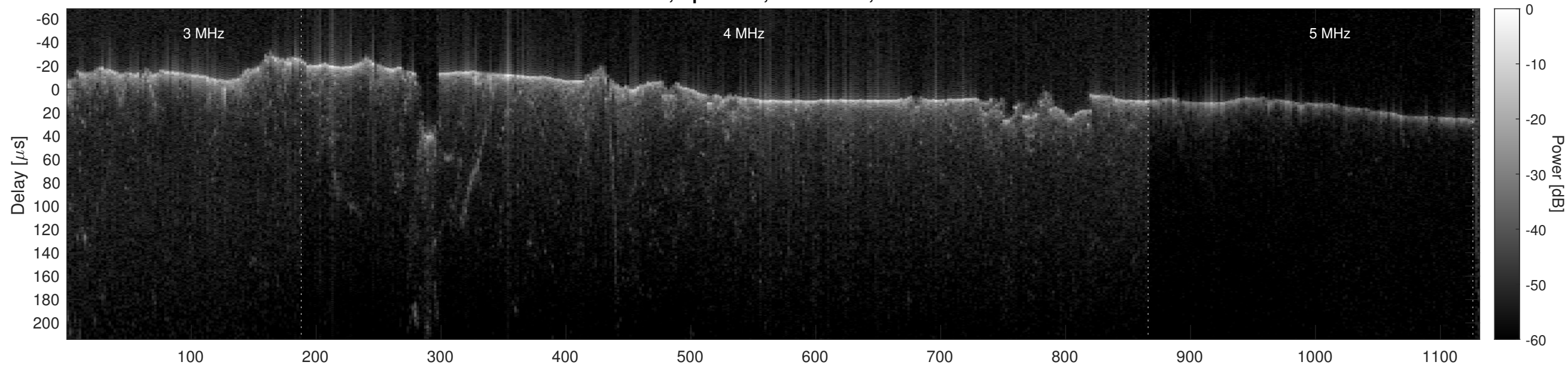
Orbit 6097, Optimized, No Window, Channel 2
