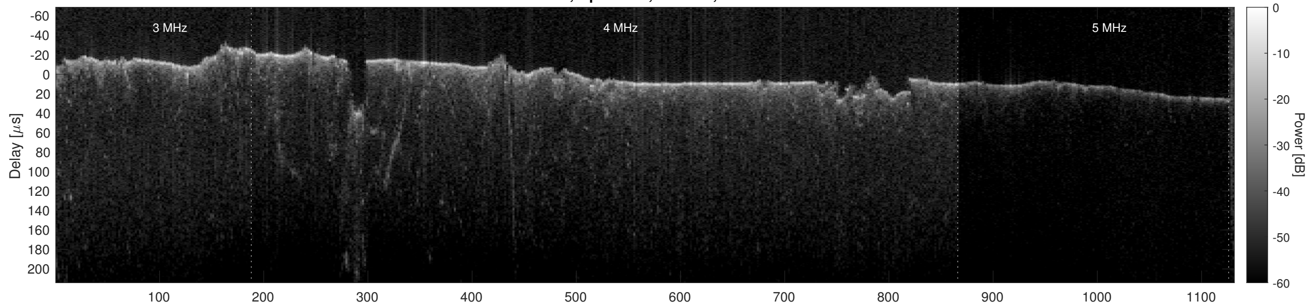
Orbit 6097, Optimized, Window, Channel 2
