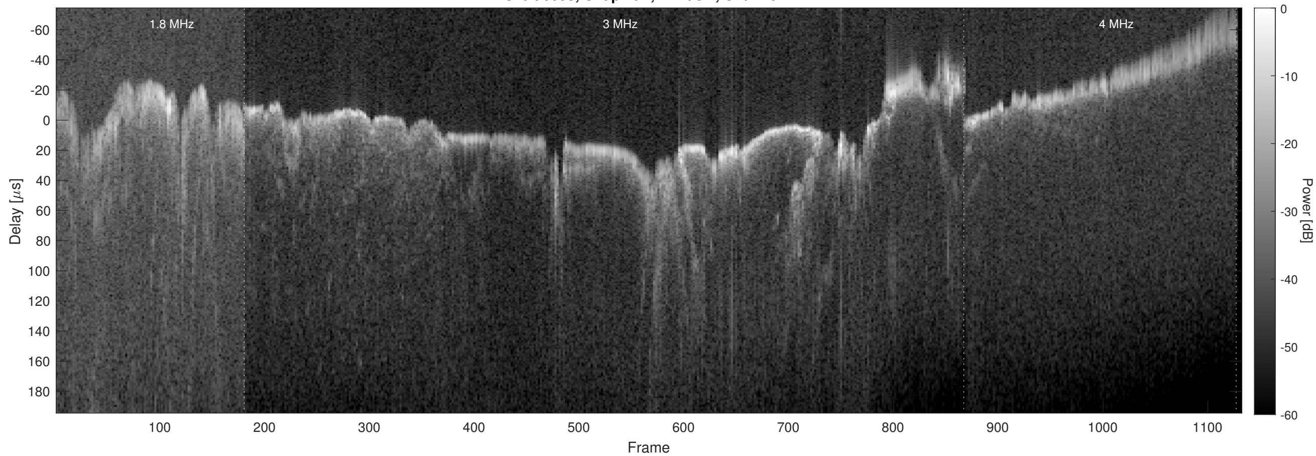
Orbit 6098, Chapman, Window, Channel 2
