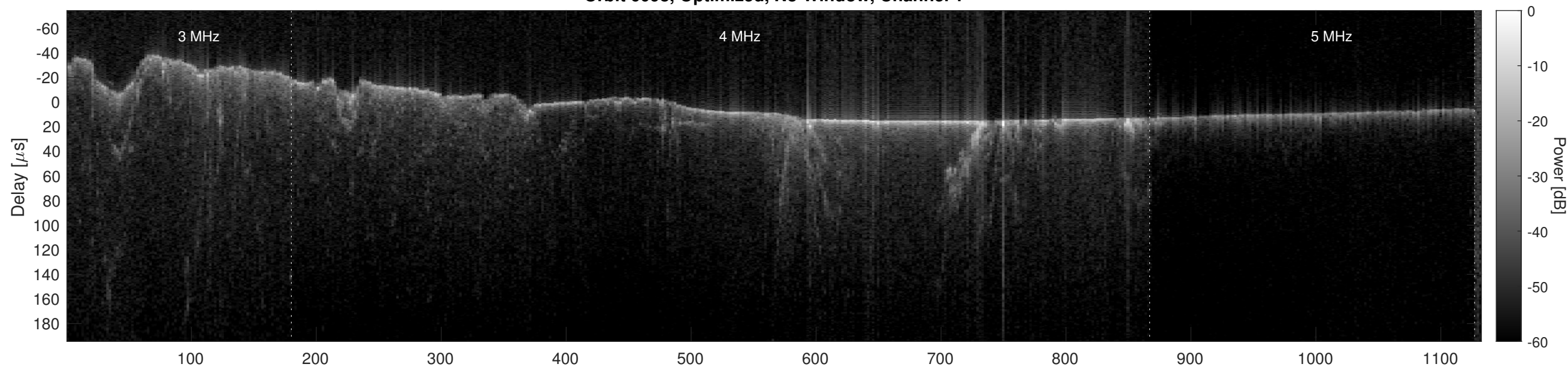
Orbit 6098, Optimized, No Window, Channel 2
