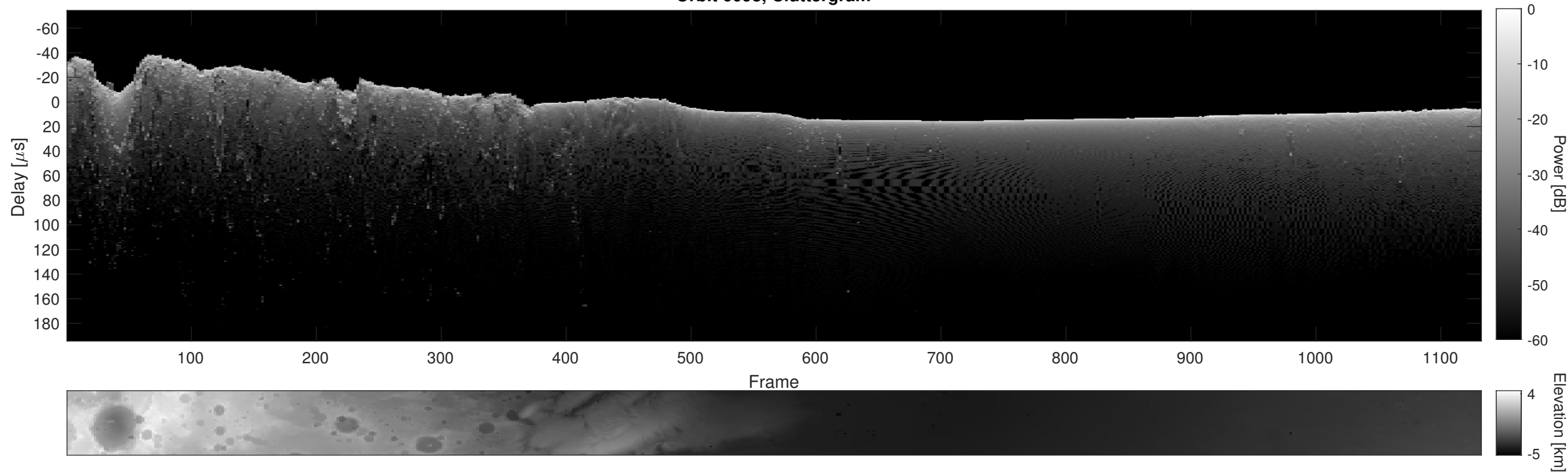
Orbit 6098, Cluttergram
