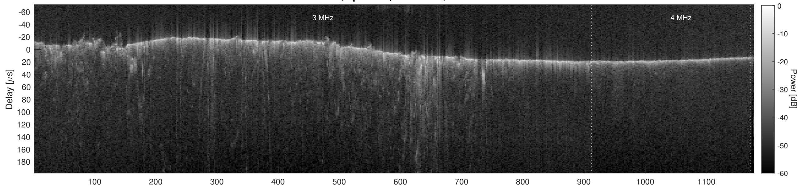
Orbit 6099, Cluttergram
