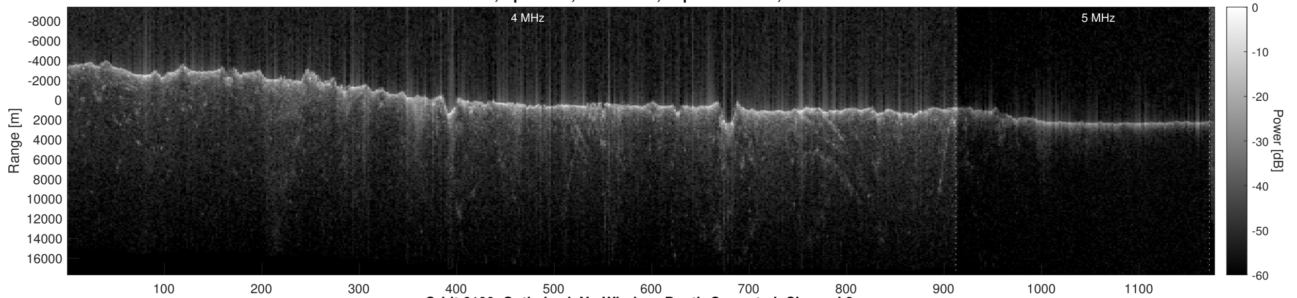
Orbit 6100, Optimized, No Window, Depth-Corrected, Channel 2
