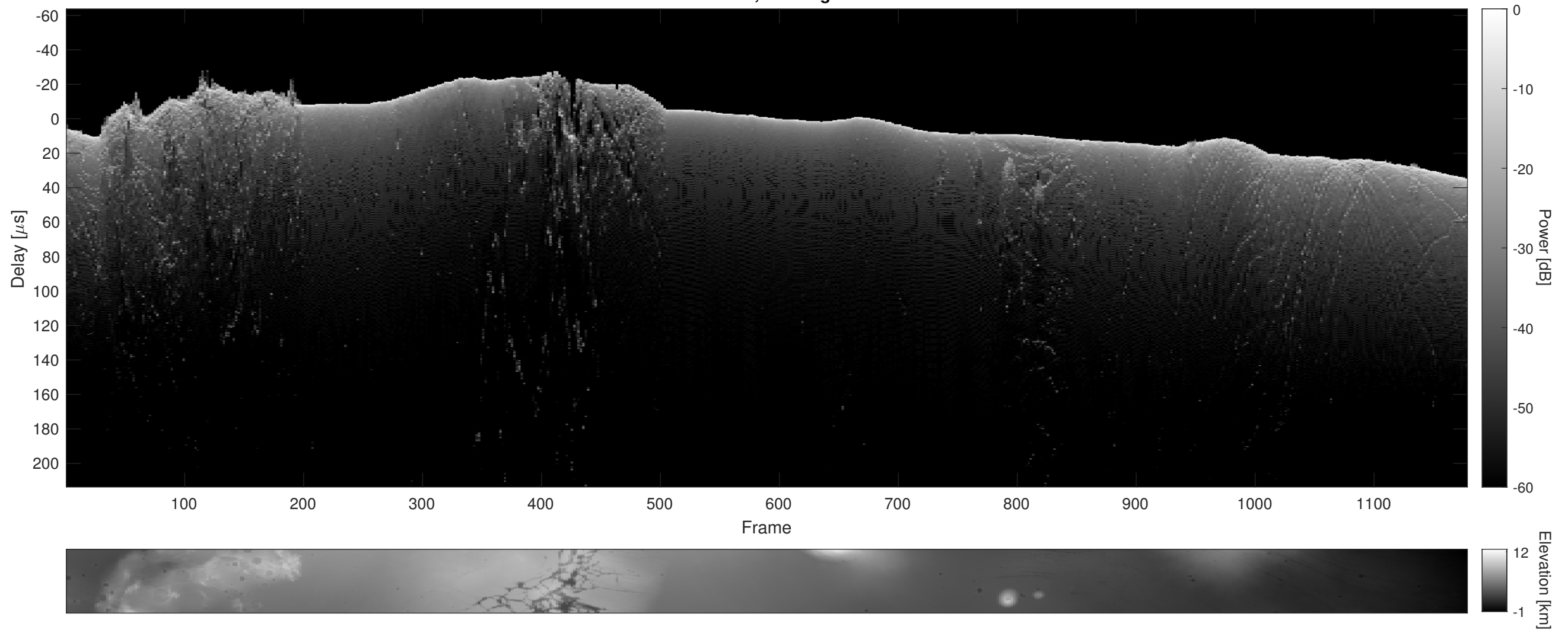
Orbit 6101, Cluttergram
