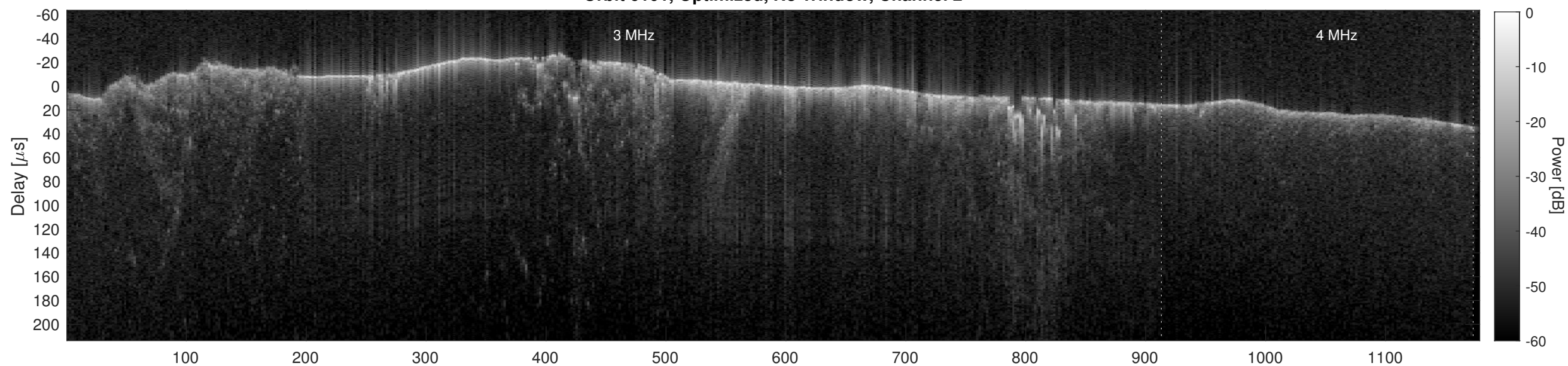
Orbit 6101, Cluttergram
