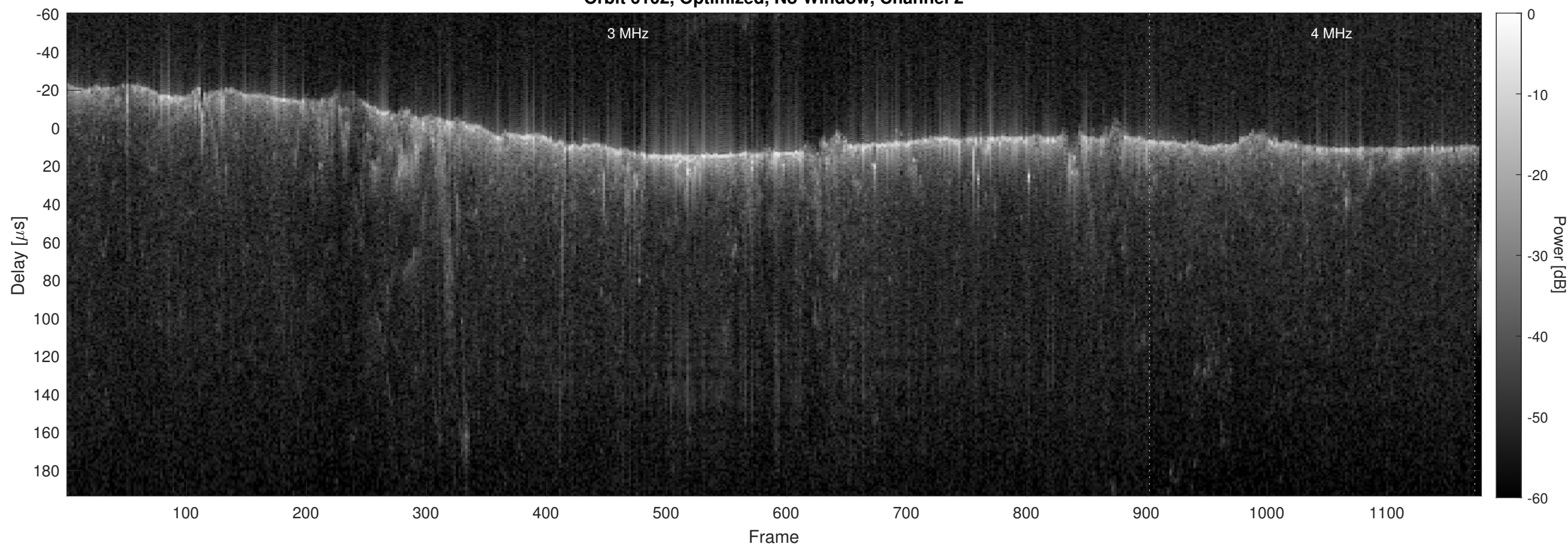
Orbit 6102, Optimized, No Window, Channel 2
