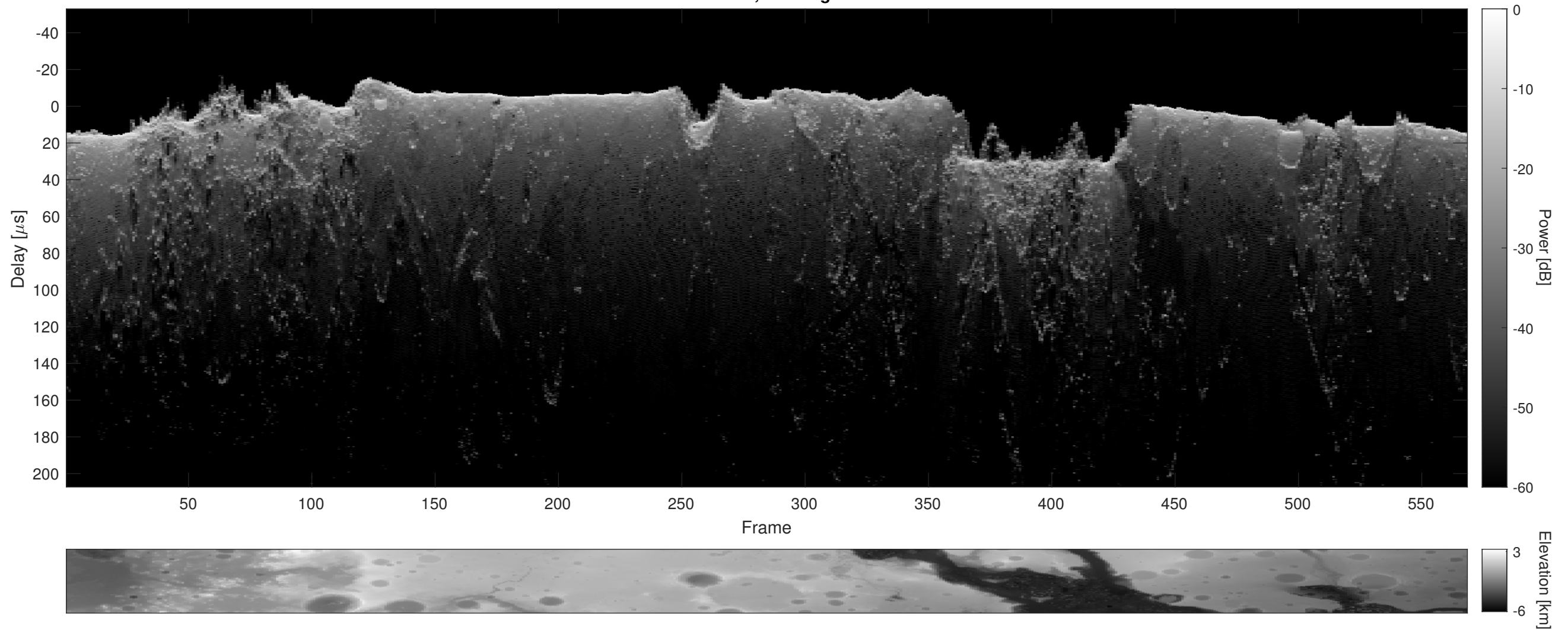
Orbit 6104, Cluttergram
