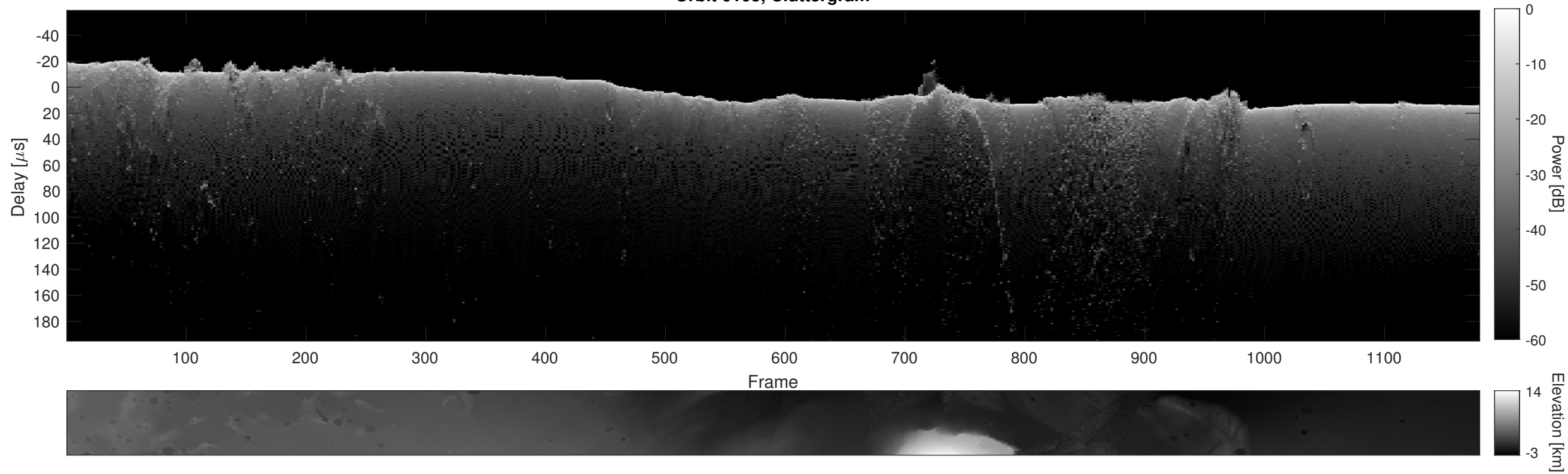
Orbit 6105, Cluttergram
