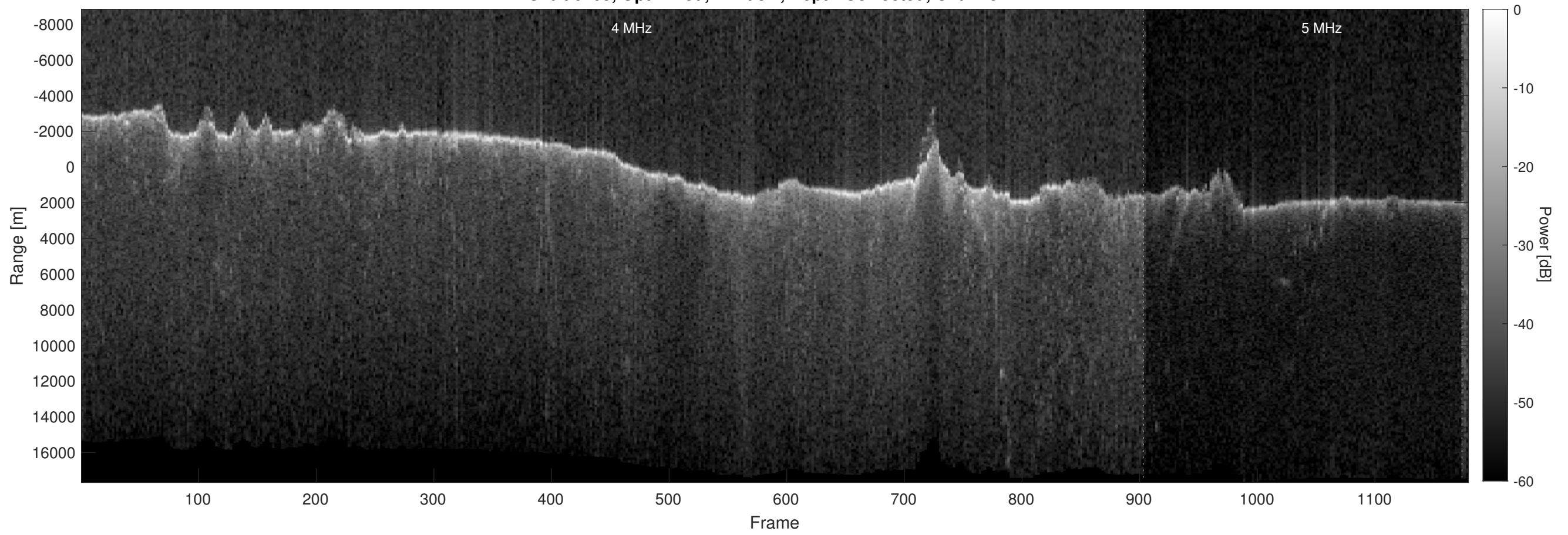
Orbit 6105, Optimized, Window, Depth-Corrected, Channel 2
