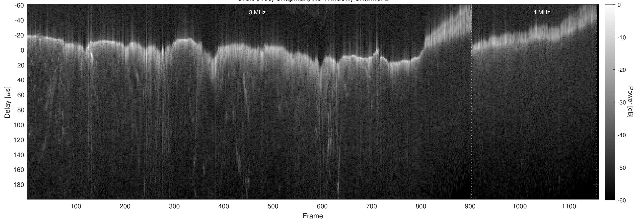
Orbit 6106, Chapman, No Window, Channel 2
