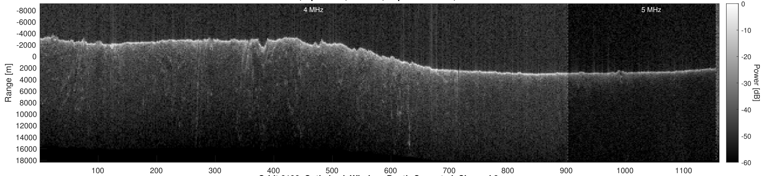
Orbit 6106, Optimized, Window, Depth-Corrected, Channel 2
