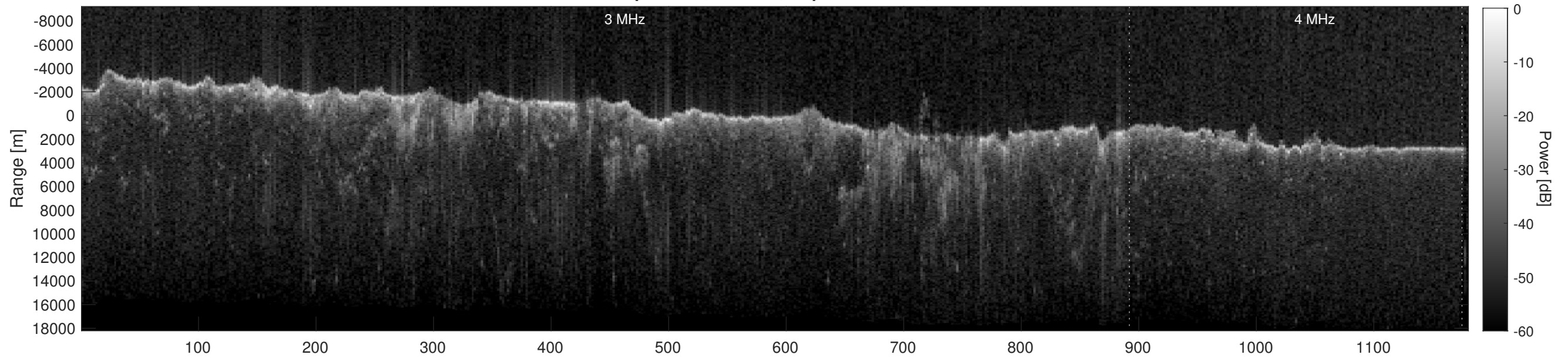
Orbit 6107, Depth-Corrected Cluttergram
