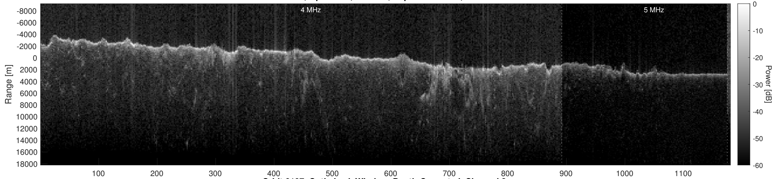
Orbit 6107, Optimized, Window, Depth-Corrected, Channel 2
