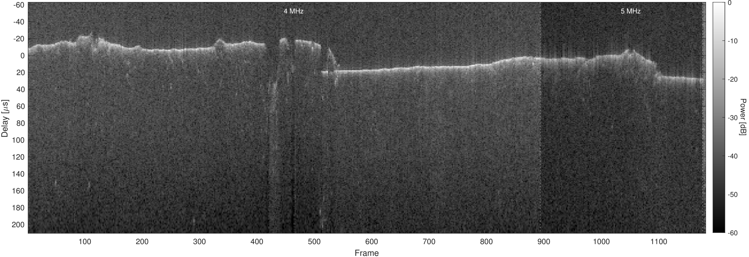
Orbit 6108, Optimized, No Window, Channel 2
