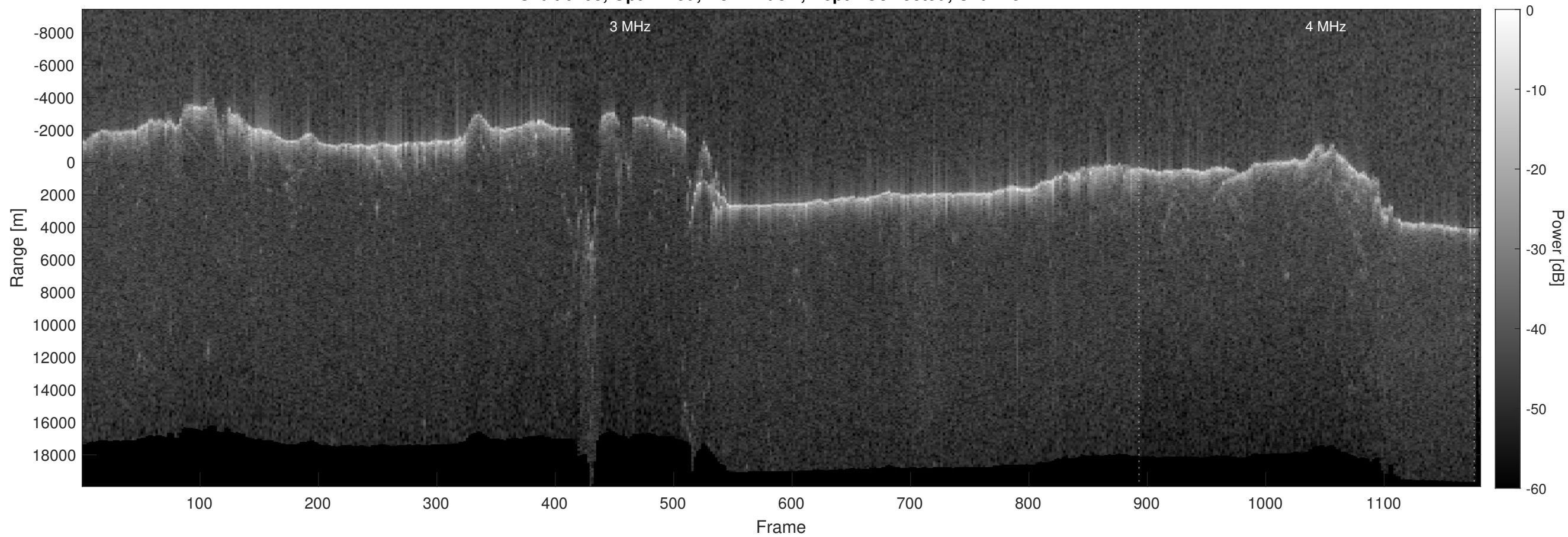
Orbit 6108, Optimized, No Window, Depth-Corrected, Channel 2
