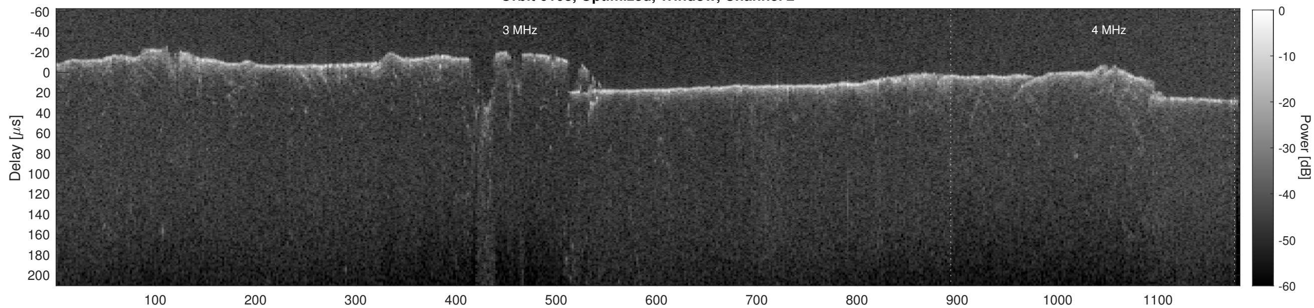
Orbit 6108, Cluttergram
