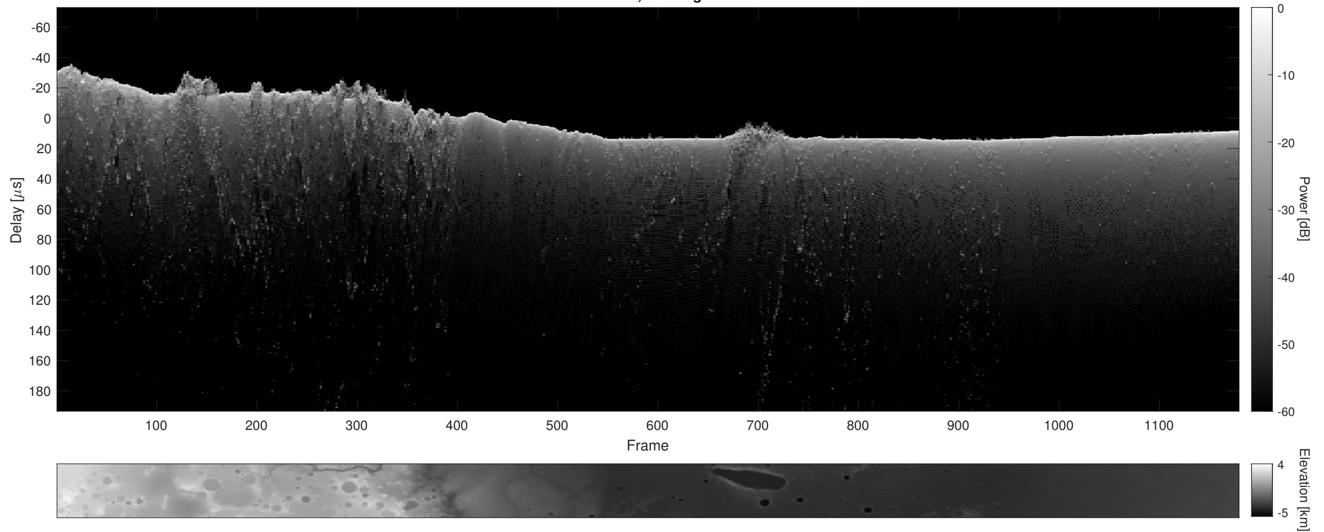
Orbit 6109, Cluttergram
