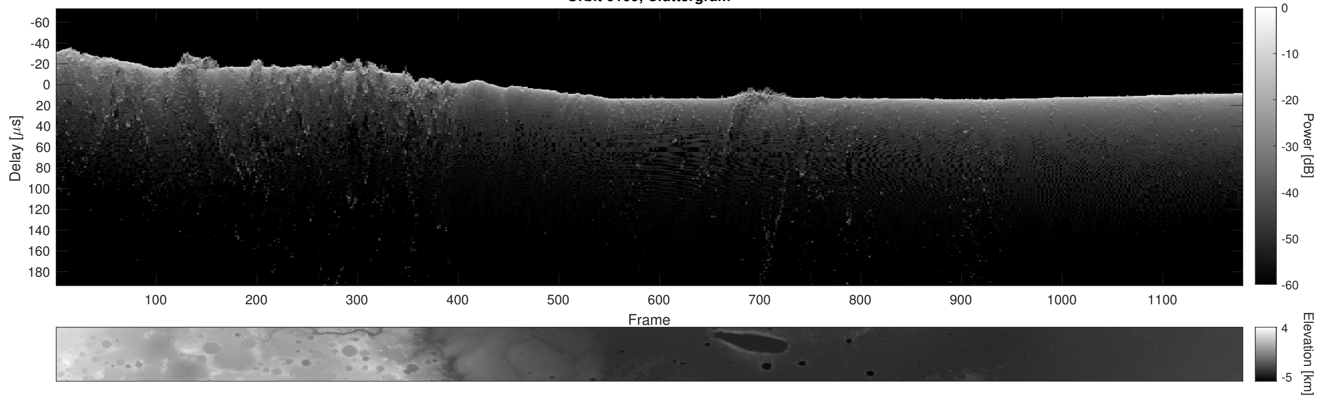
Orbit 6109, Cluttergram
