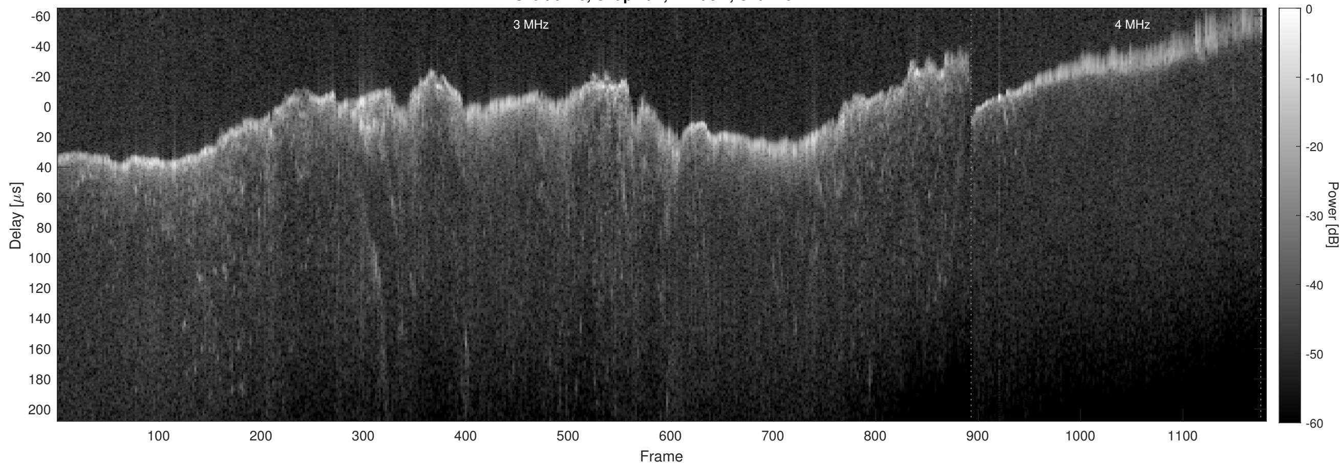
Orbit 6110, Chapman, Window, Channel 2
