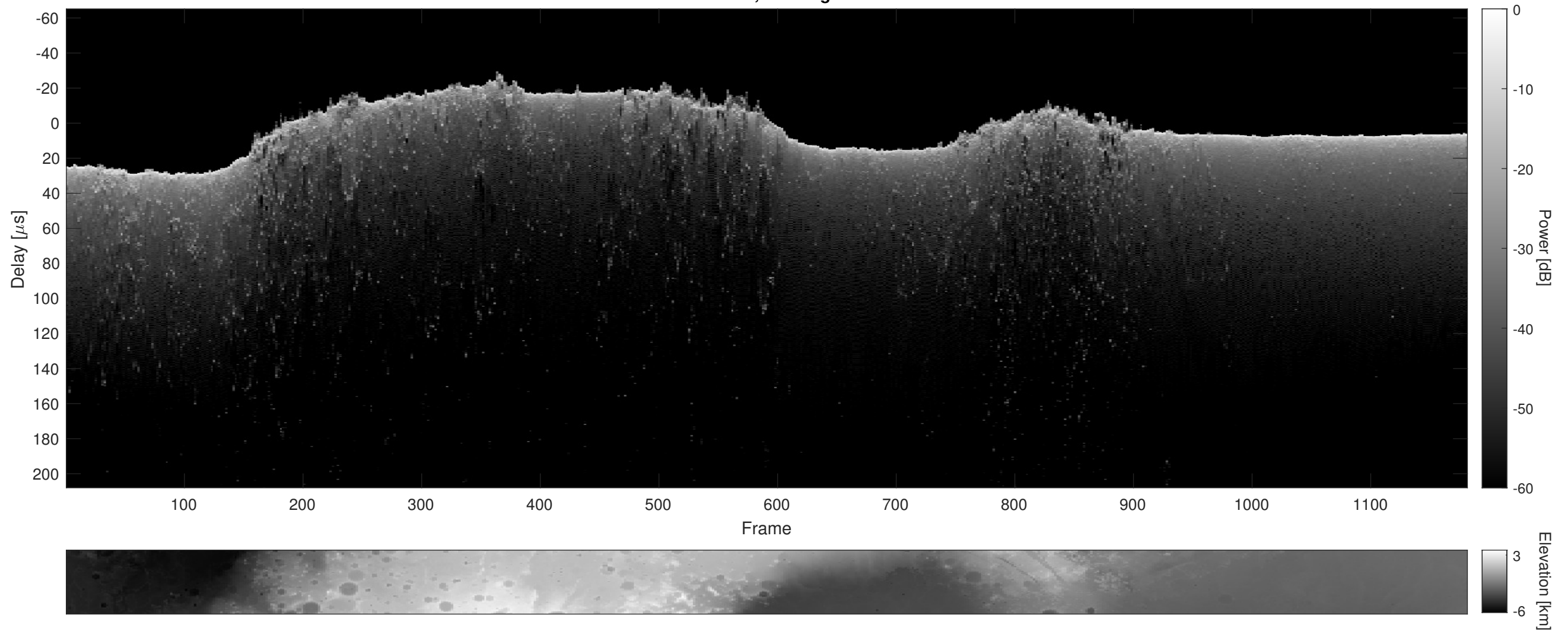
Orbit 6110, Cluttergram
