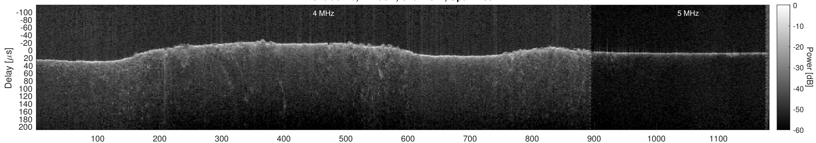
Orbit 6110, Cluttergram
