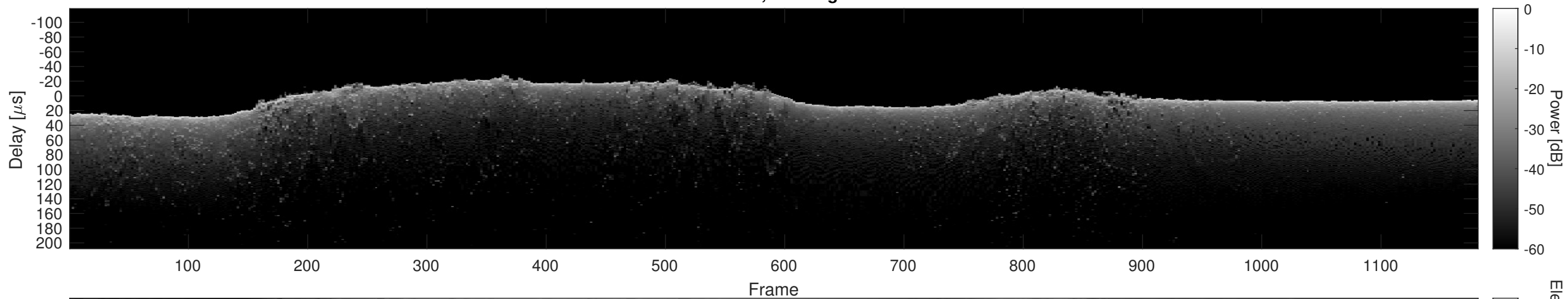
Orbit 6110, Cluttergram
