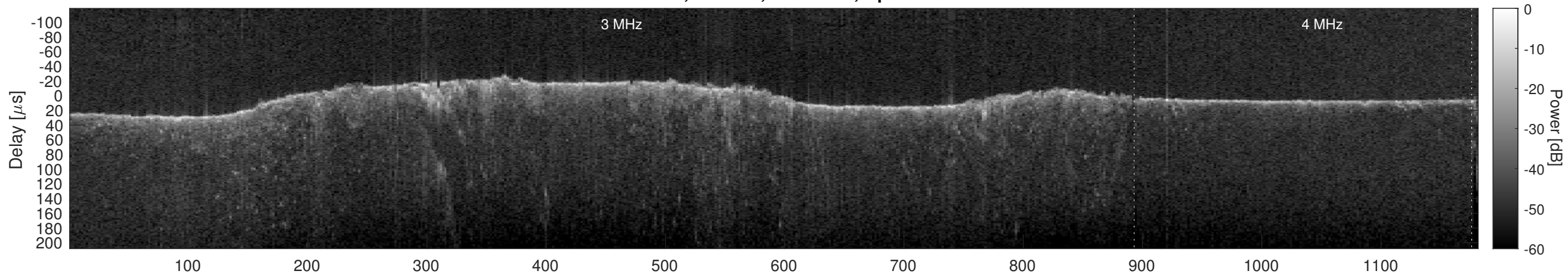
Orbit 6110, Cluttergram
