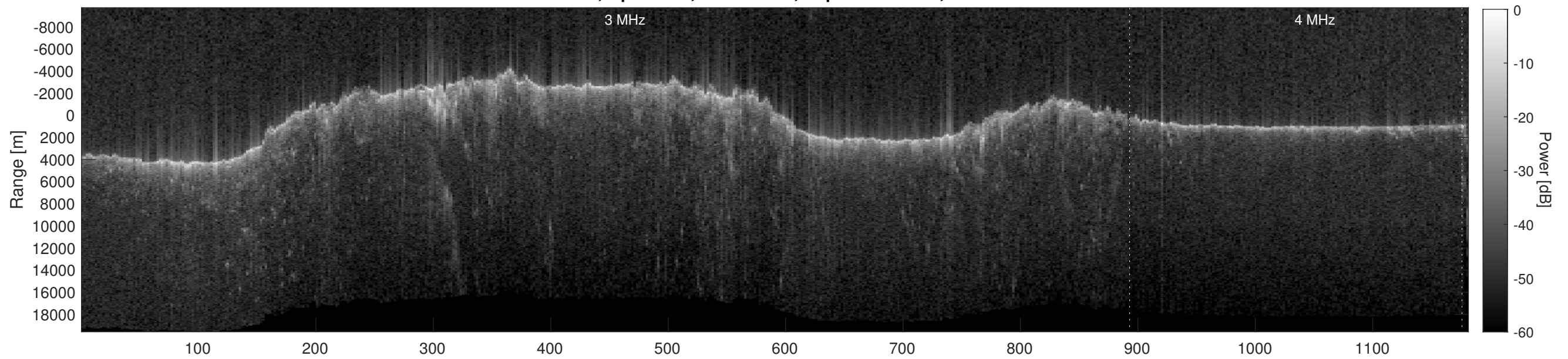
Orbit 6110, Depth-Corrected Cluttergram
