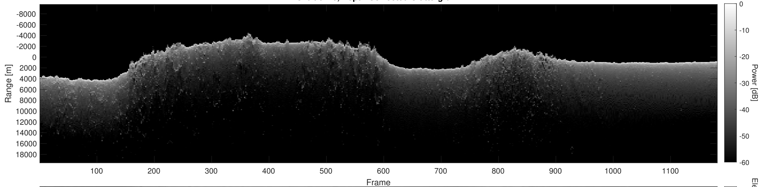
Orbit 6110, Depth-Corrected Cluttergram
