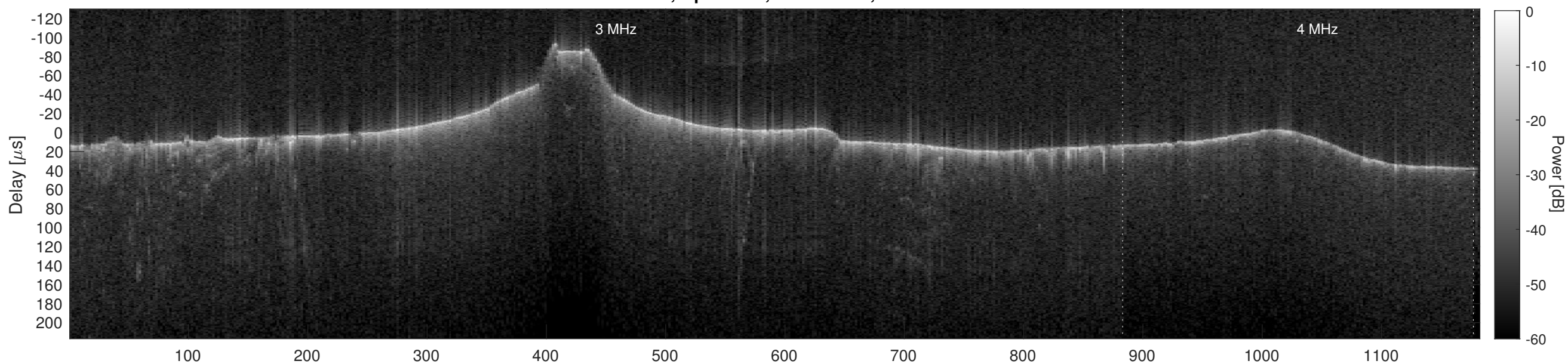
Orbit 6112, Cluttergram
