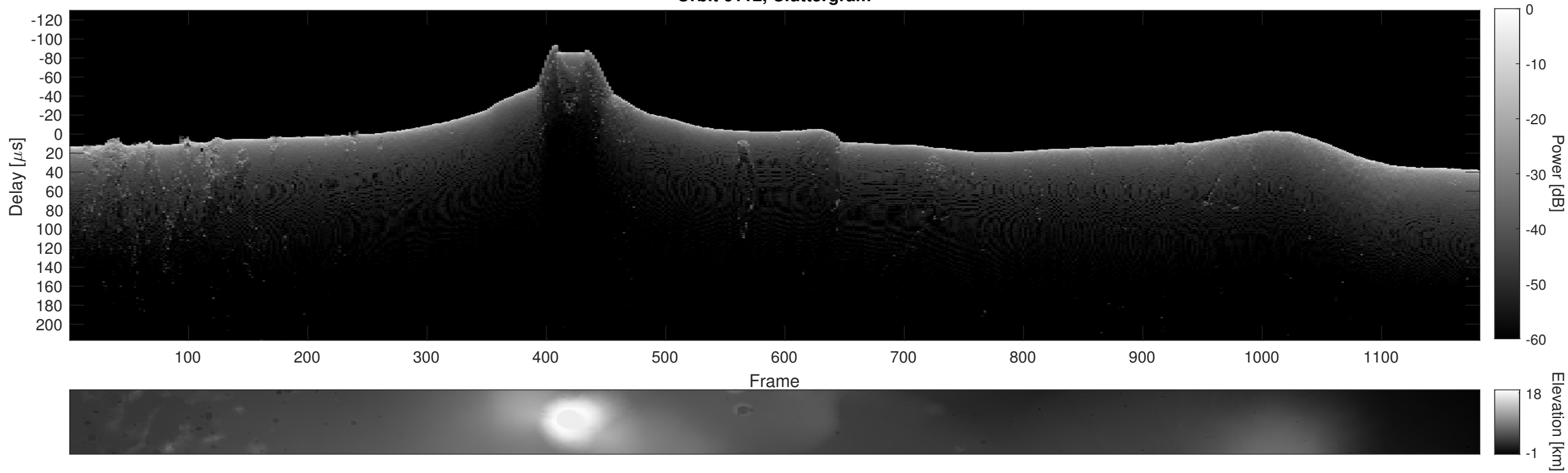
Orbit 6112, Cluttergram
