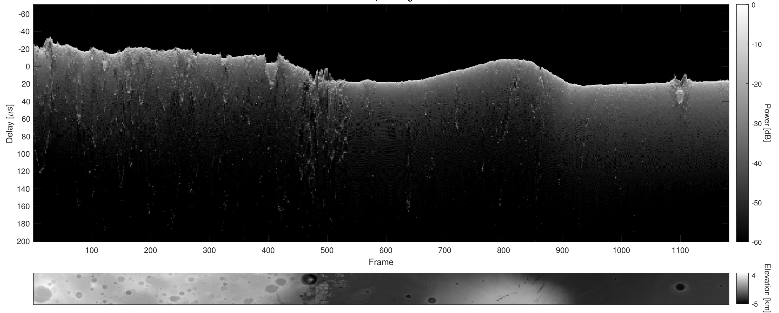
Orbit 6113, Cluttergram
