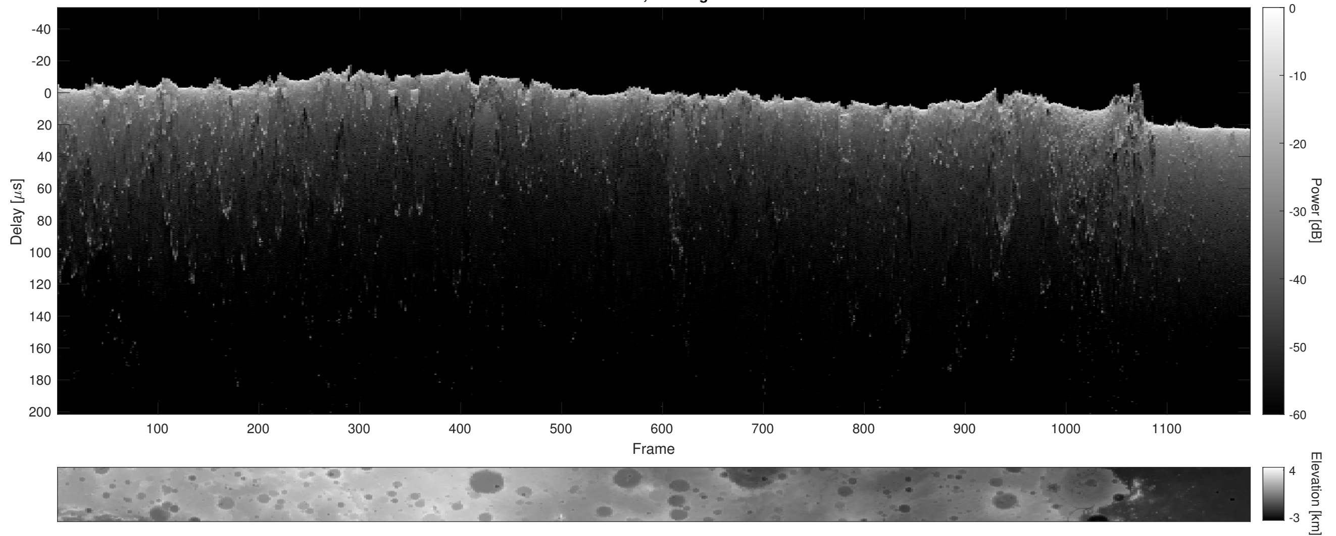
Orbit 6114, Cluttergram
