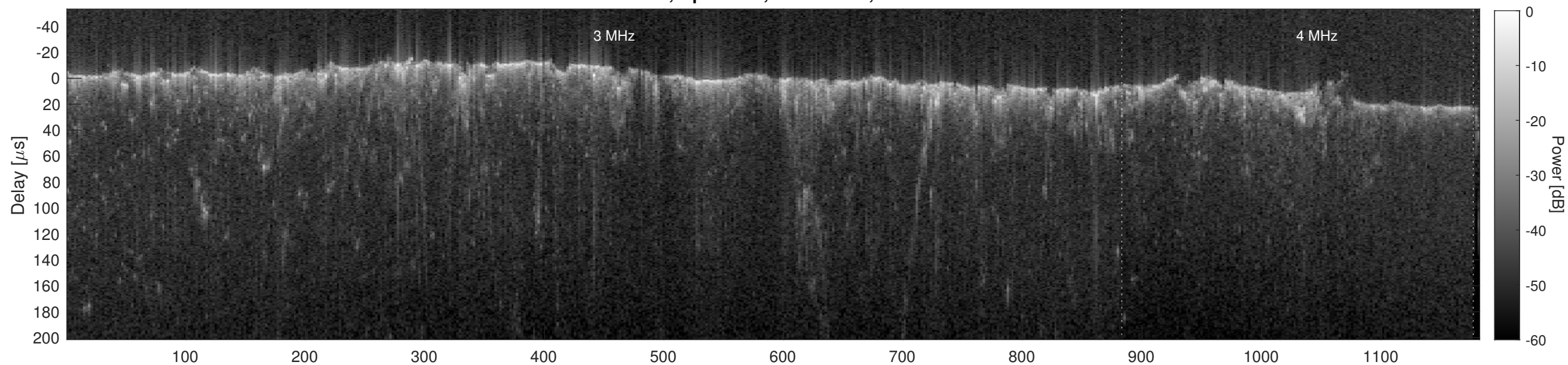
Orbit 6114, Cluttergram
