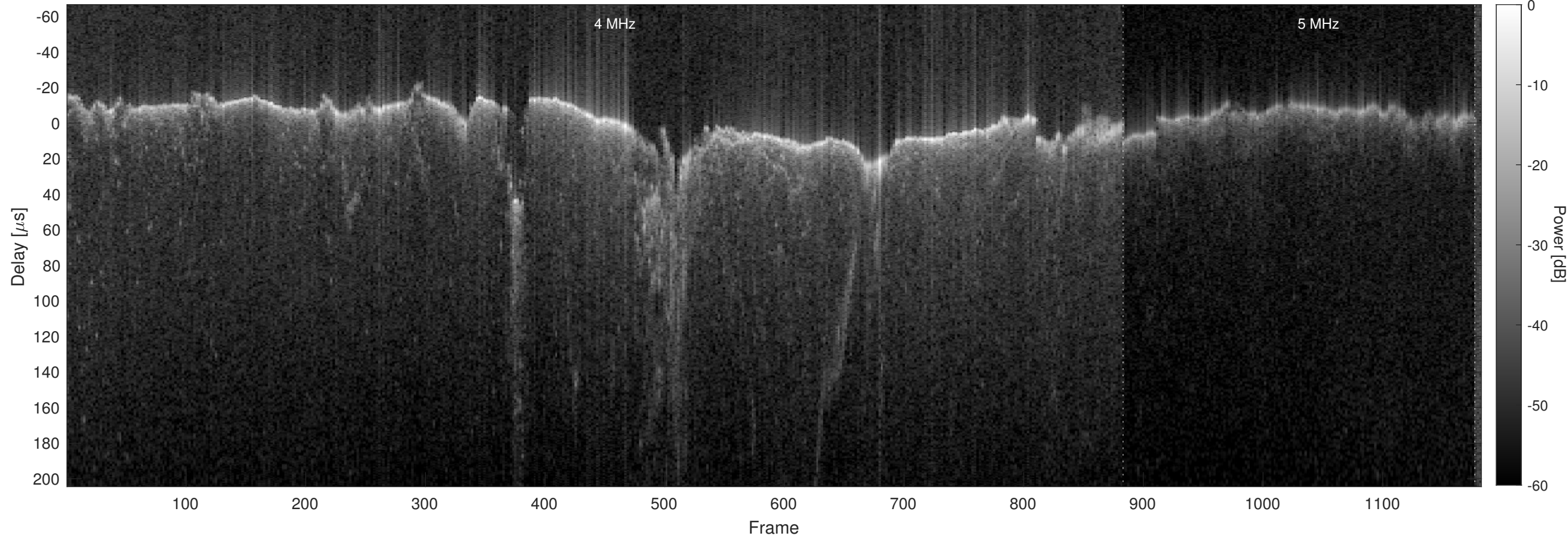
Orbit 6115, Chapman, No Window, Channel 2
