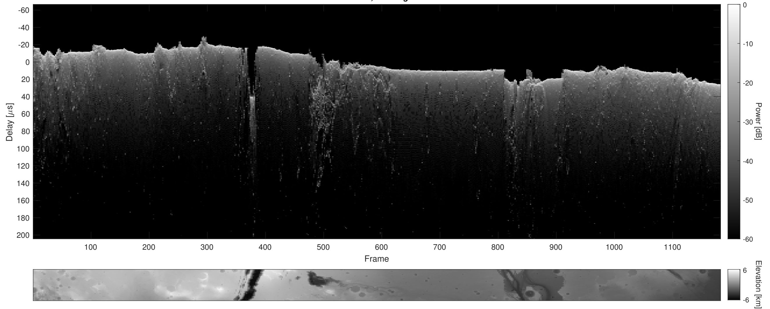
Orbit 6115, Cluttergram
