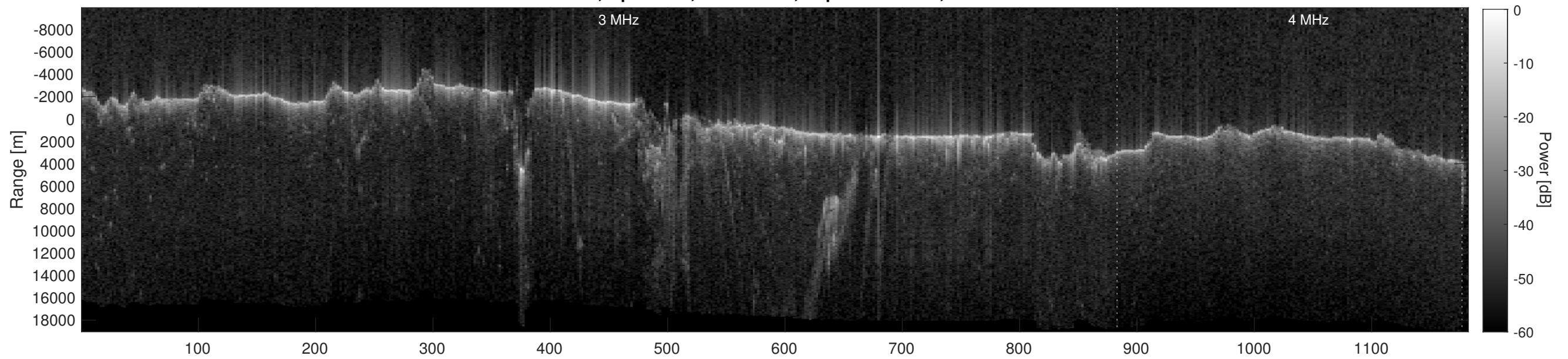
Orbit 6115, Depth-Corrected Cluttergram
