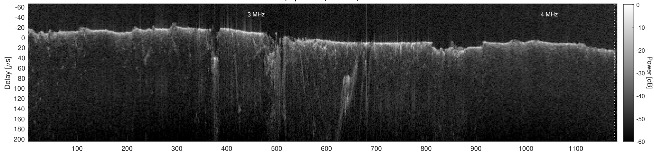
Orbit 6115, Cluttergram
