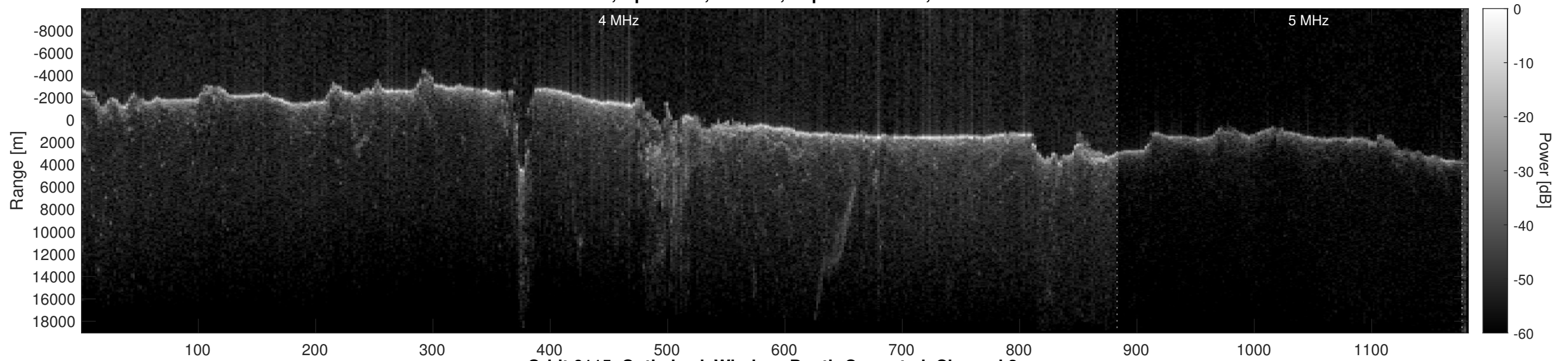
Orbit 6115, Optimized, Window, Depth-Corrected, Channel 2
