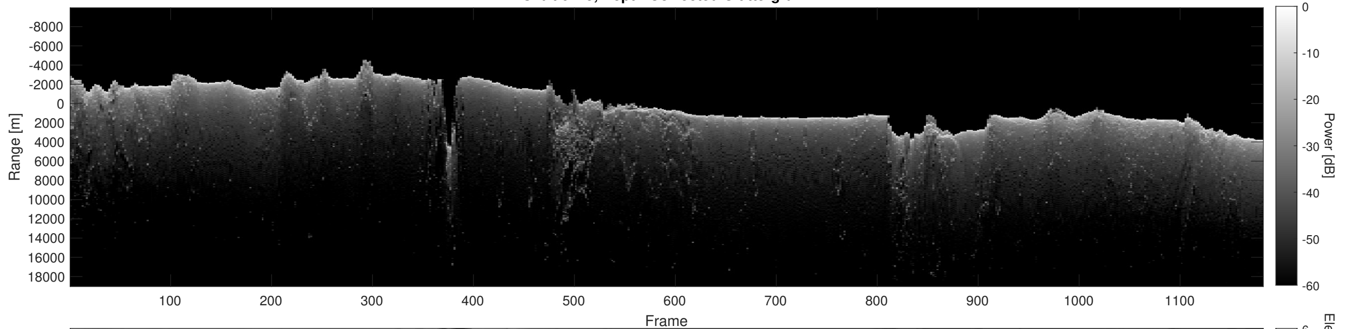
Orbit 6115, Depth-Corrected Cluttergram
