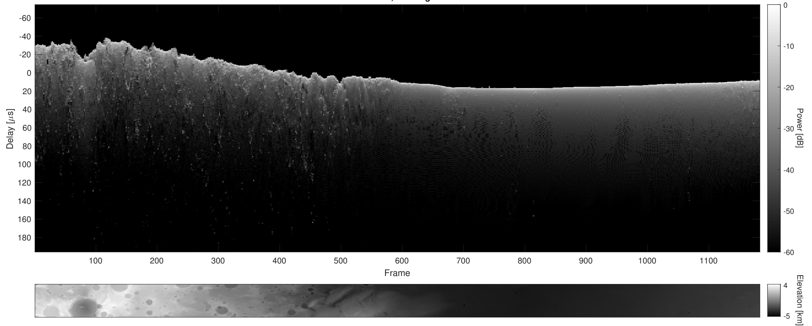
Orbit 6116, Cluttergram
