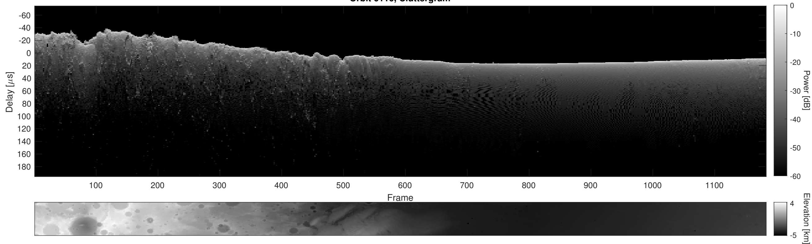
Orbit 6116, Cluttergram
