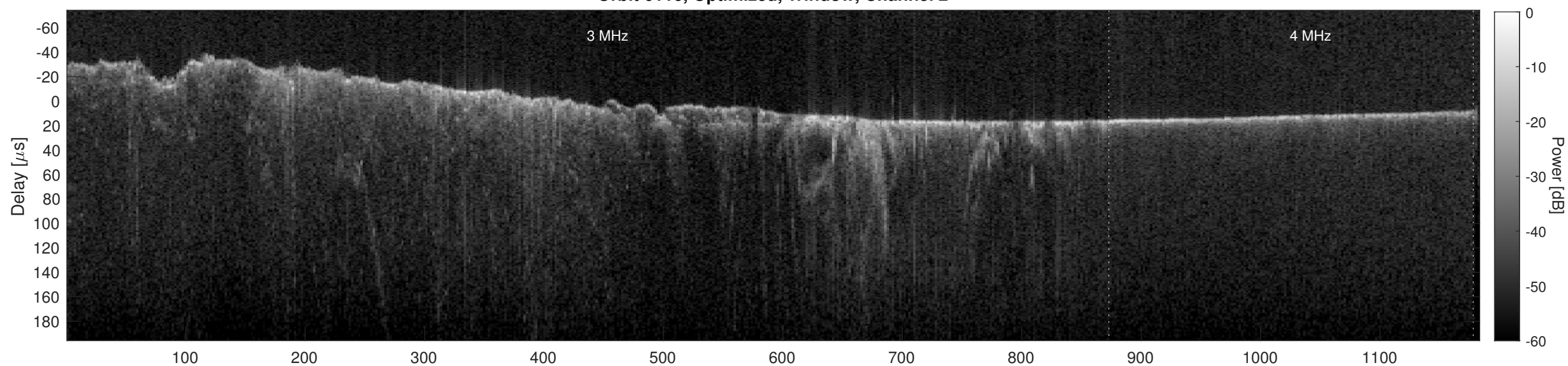
Orbit 6116, Cluttergram
