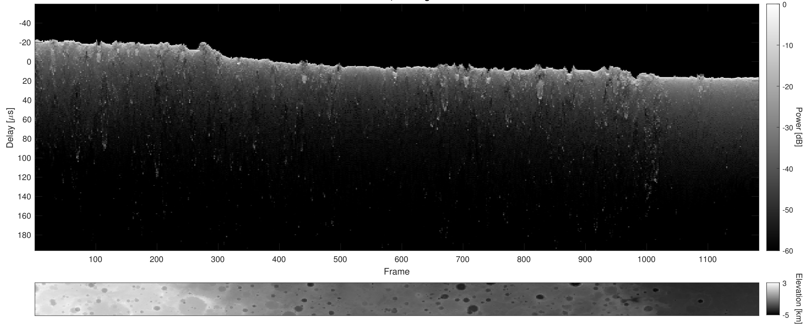
Orbit 6118, Cluttergram
