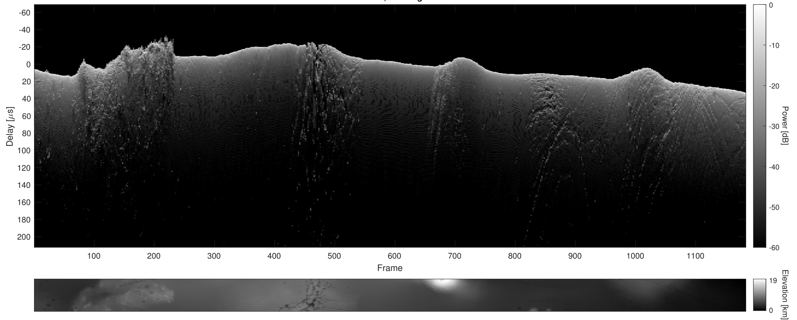
Orbit 6119, Cluttergram
