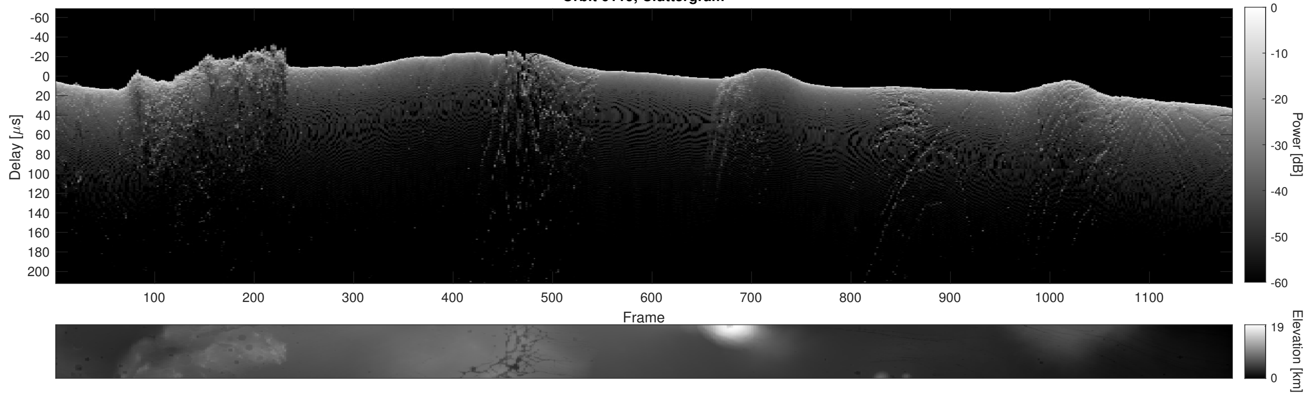
Orbit 6119, Cluttergram
