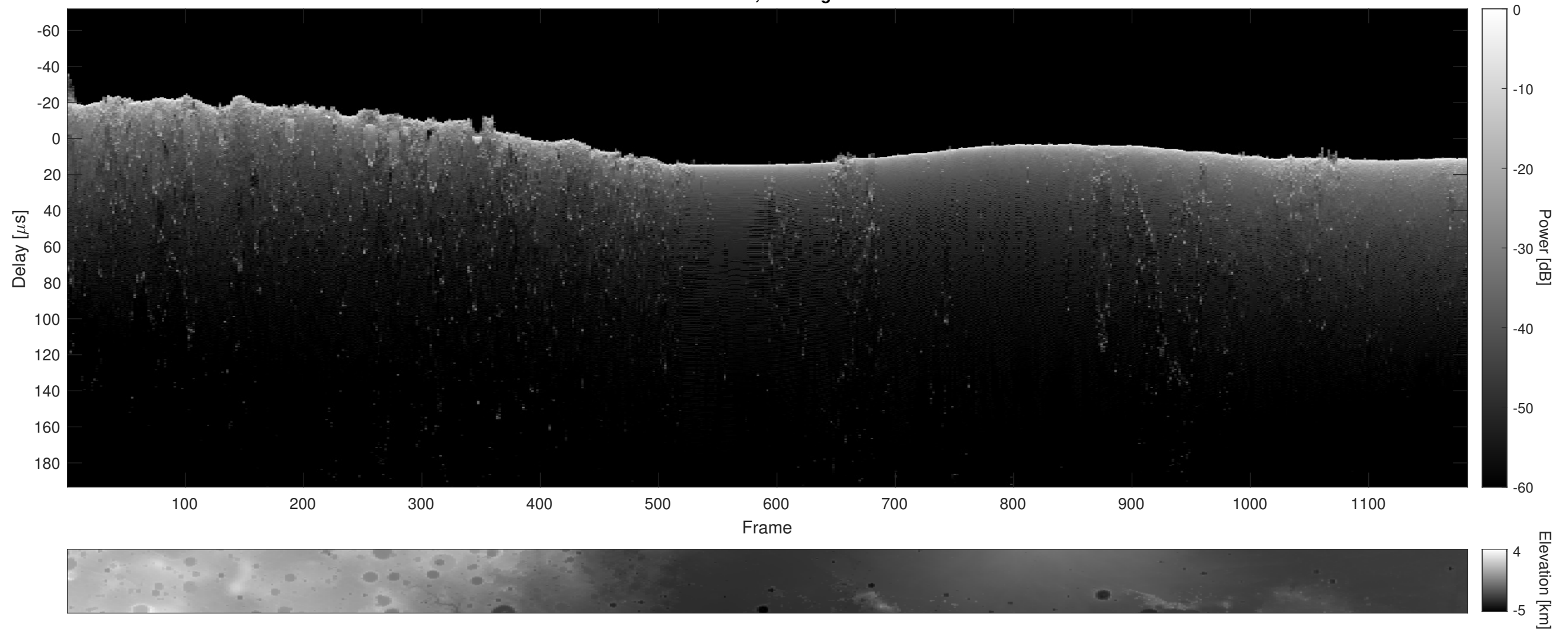
Orbit 6120, Cluttergram
