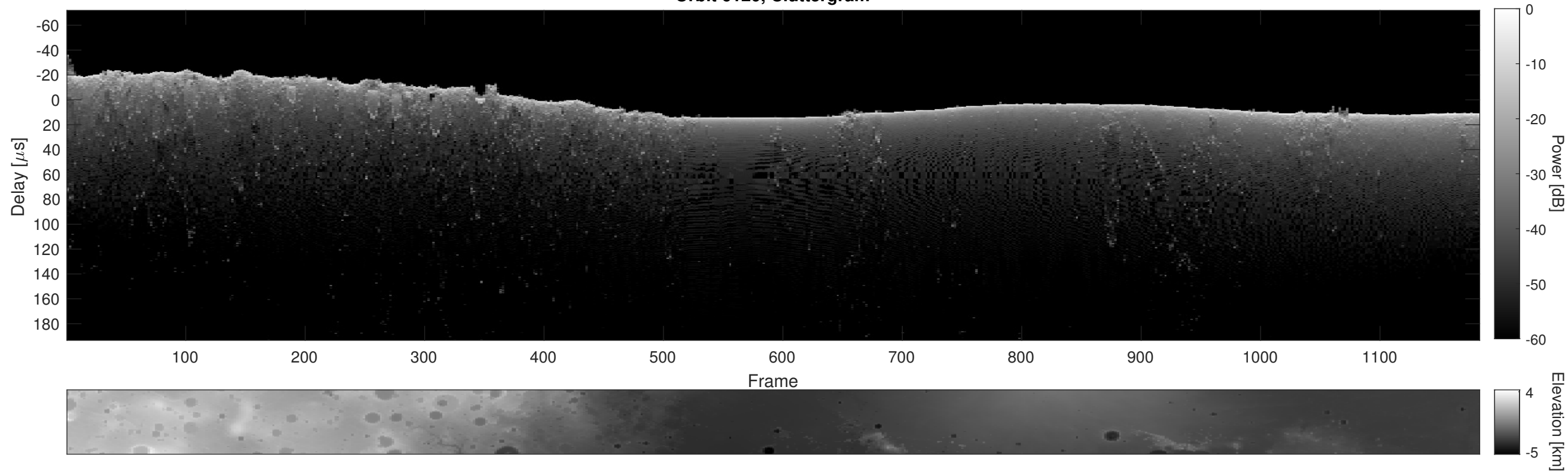
Orbit 6120, Cluttergram
