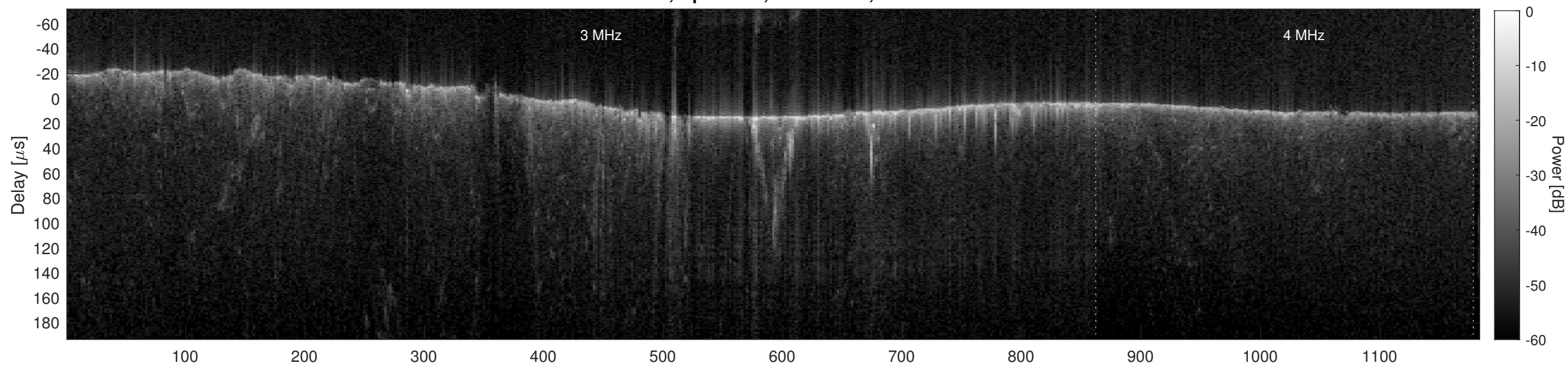
Orbit 6120, Cluttergram
