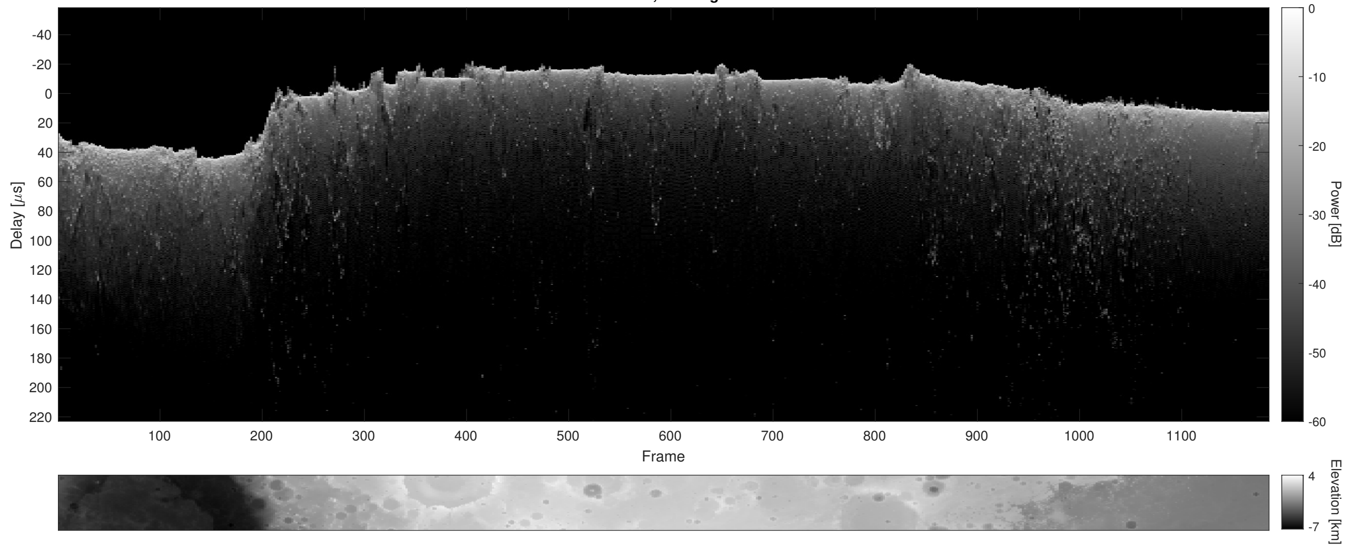
Orbit 6121, Cluttergram
