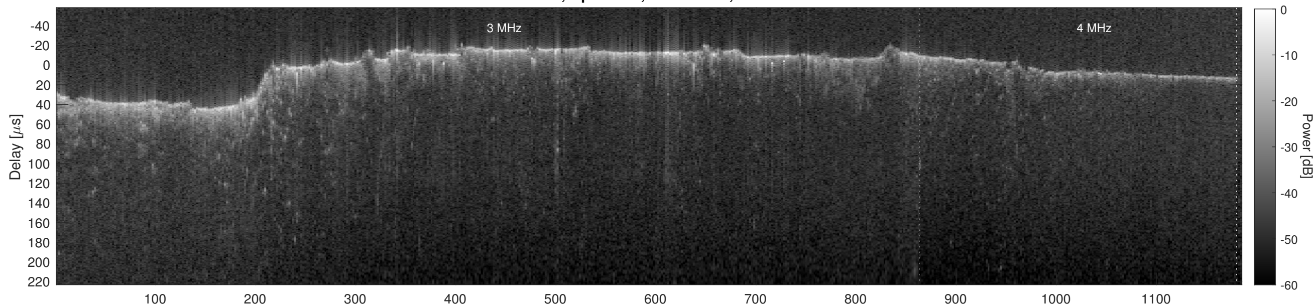
Orbit 6121, Cluttergram
