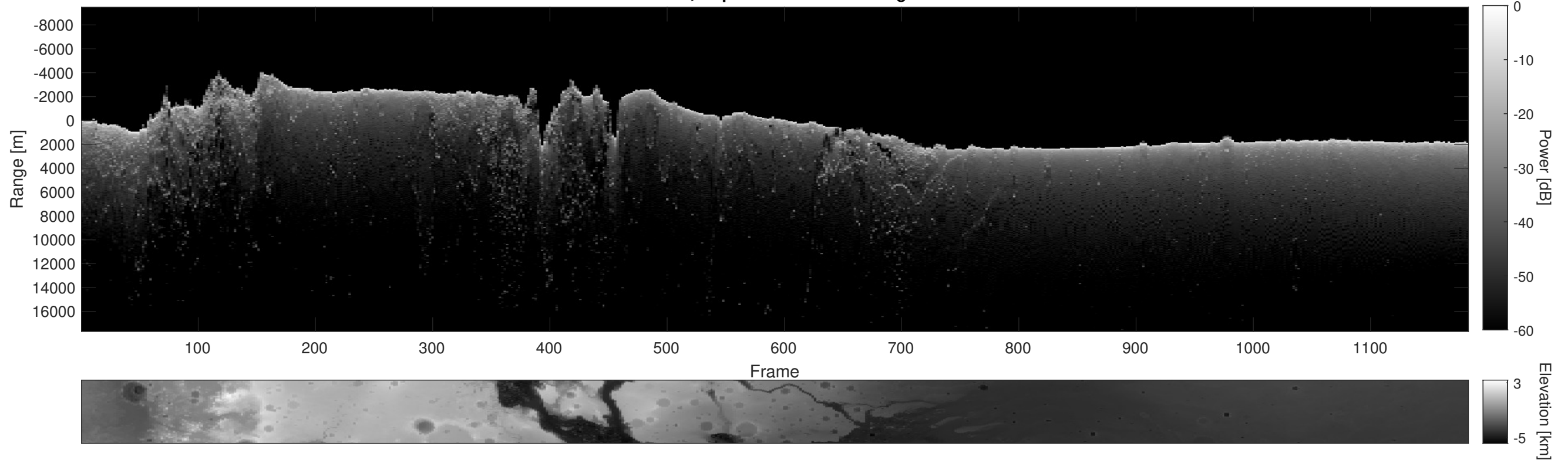
Orbit 6122, Depth-Corrected Cluttergram
