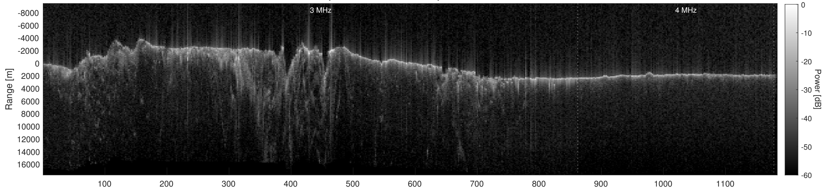
Orbit 6122, Depth-Corrected Cluttergram
