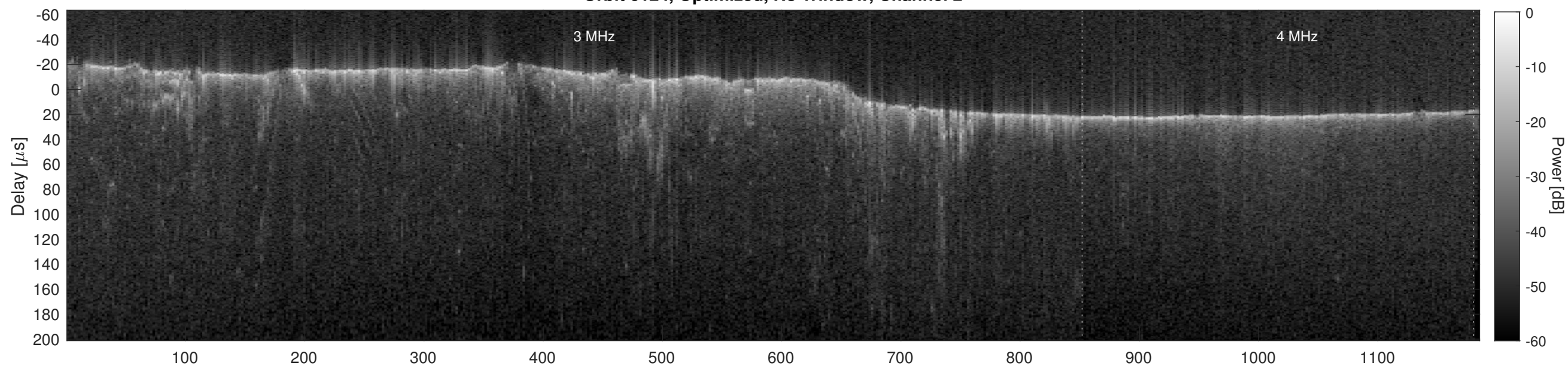
Orbit 6124, Cluttergram
