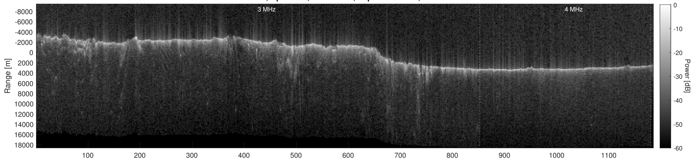
Orbit 6124, Depth-Corrected Cluttergram
