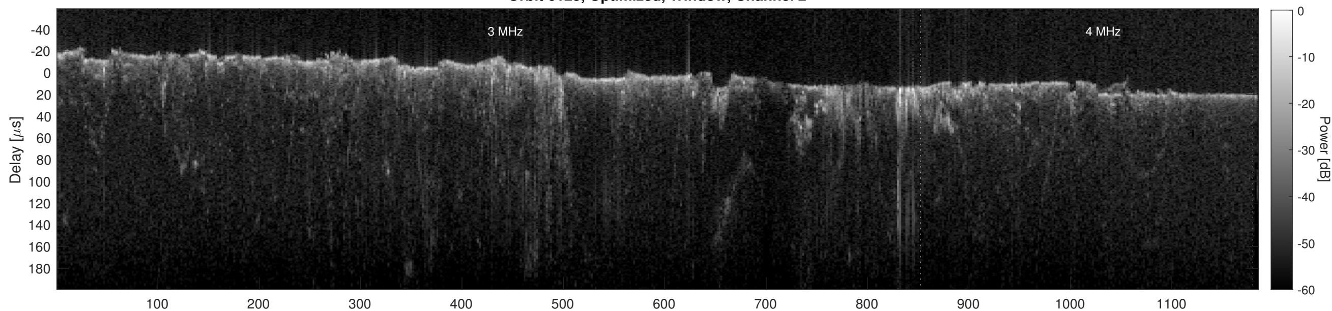
Orbit 6125, Cluttergram
