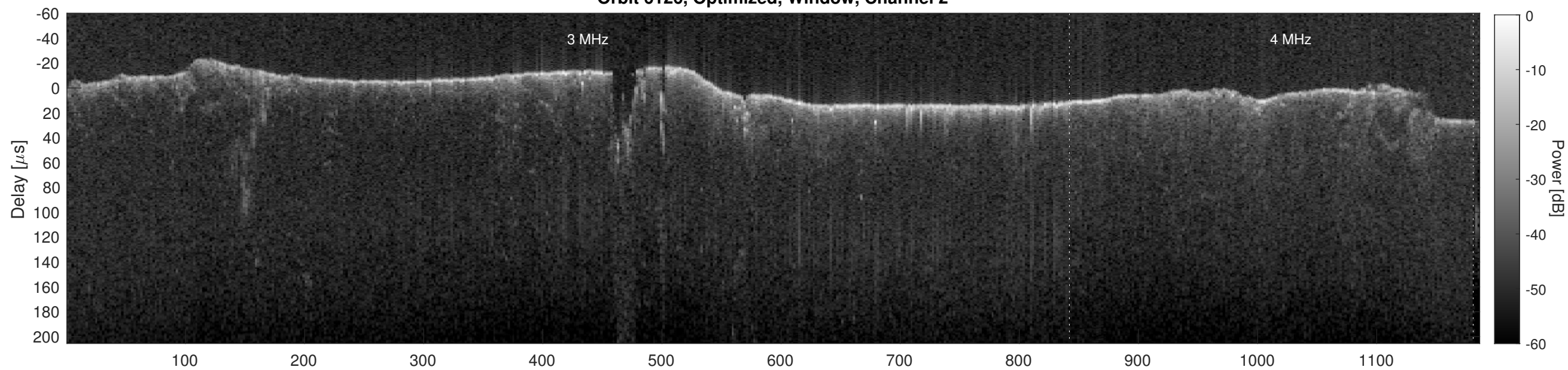
Orbit 6126, Cluttergram
